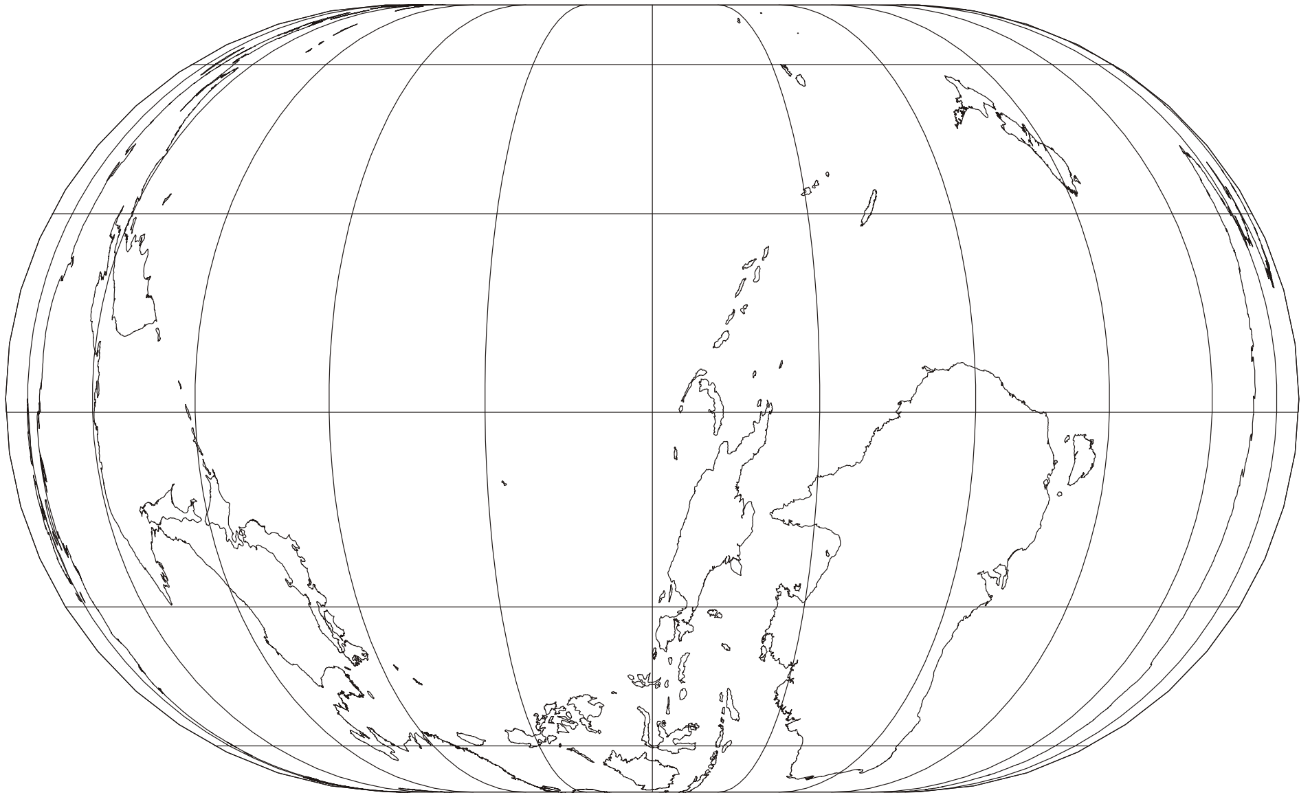
Maurer SNo. 196 (Double Retroazimuthal) projection; Retroazimuthal; Neither Conformal nor Equal-area; Hans Maurer; 1911
