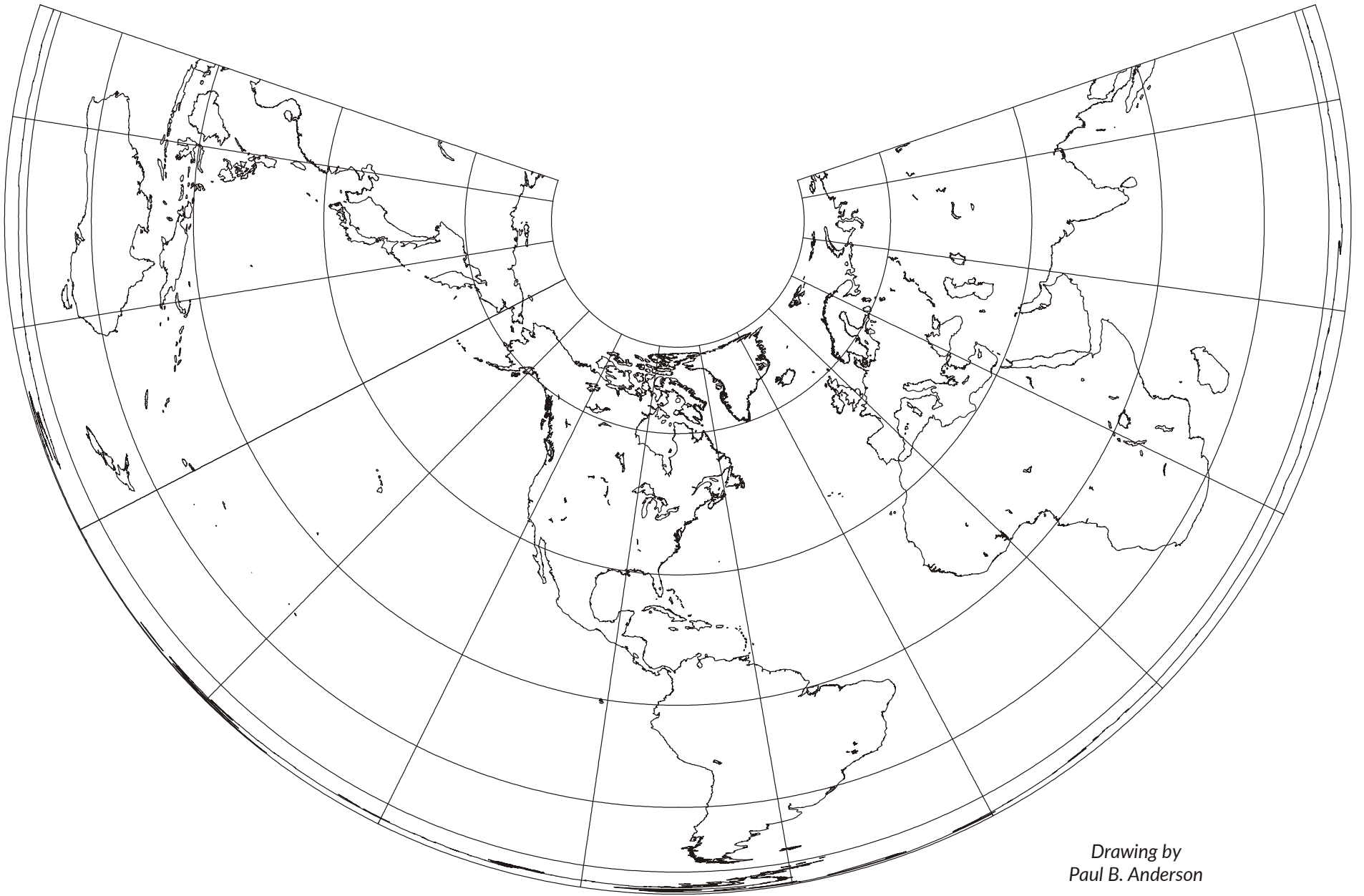
Albers Equal-area Conic; H. C. Albers; 1805
