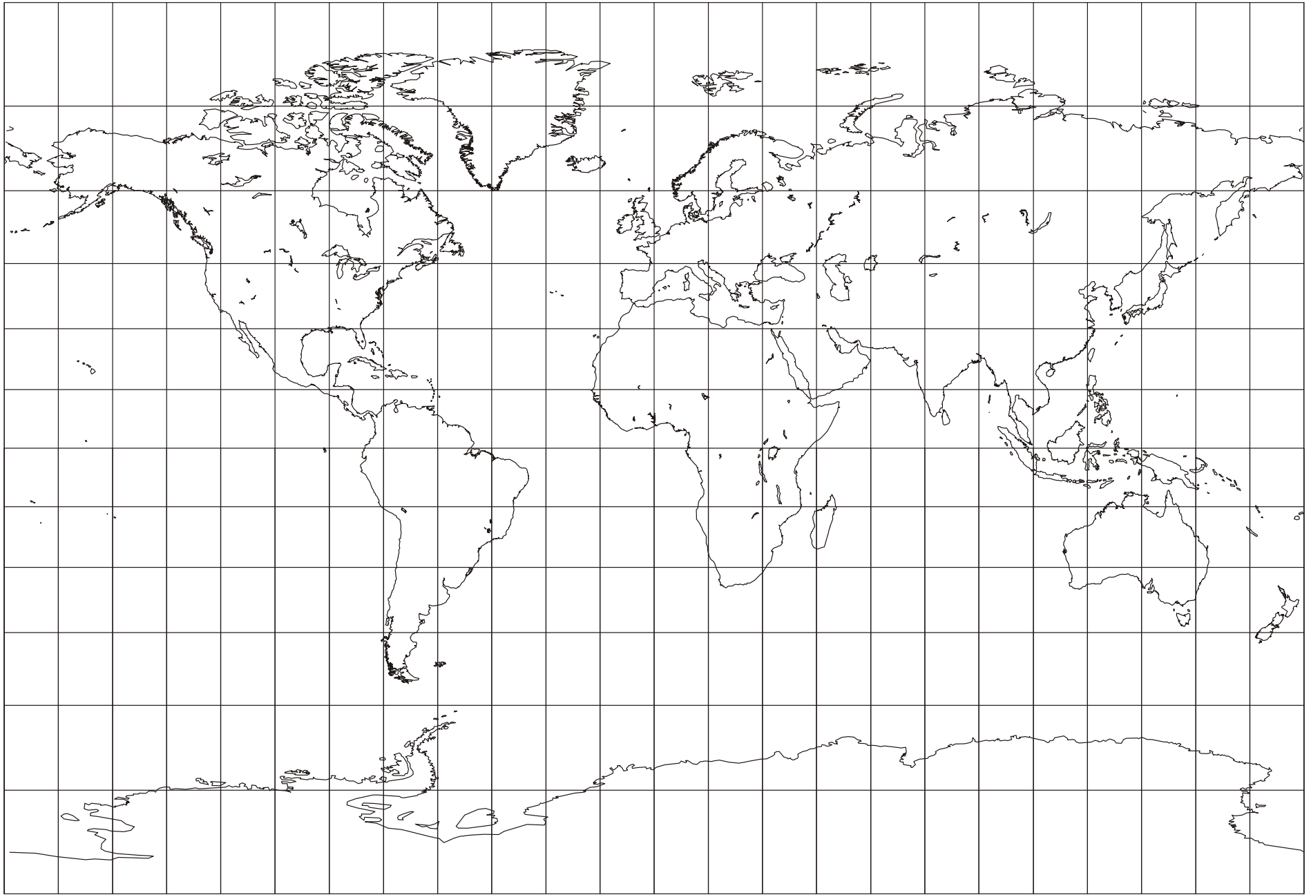
BSAM Cylindrical (Modified Gall Stereographic); Standard Parallels = 30 Deg.; Neither Conformal or Equal-area; V. A. Kamenetskiy; 1937
