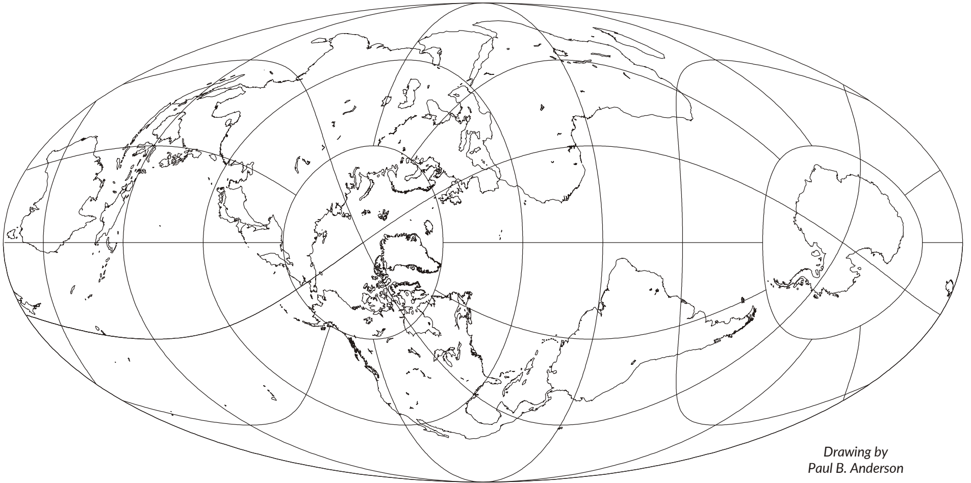
Atlantis projection; (Transverse Mollweide); Pseudocylindrical; Equal-area; John Bartholomew; 1948
