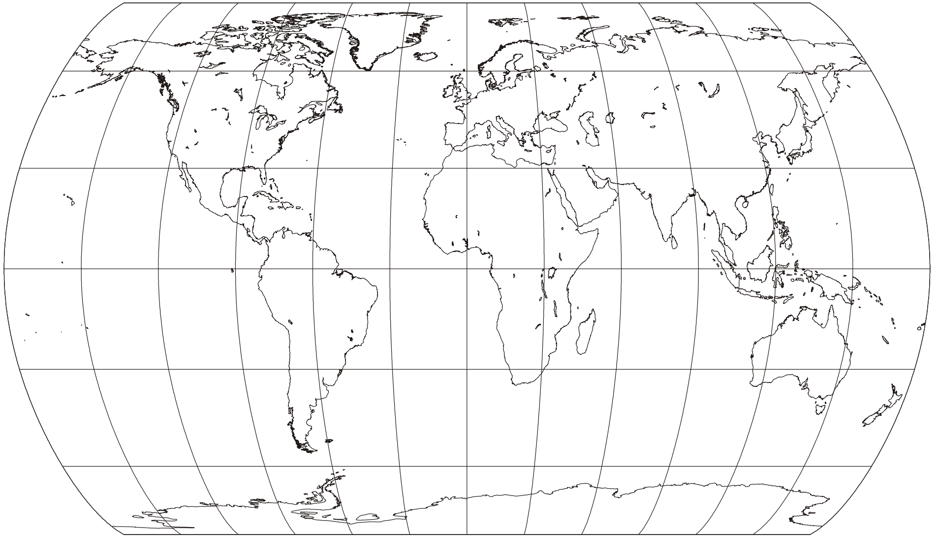
Canters Low-error Pseudocylindrical (a) projection; (With twofold symmetry); Neither Conformal or Equal-area; Frank Canters; 2002
