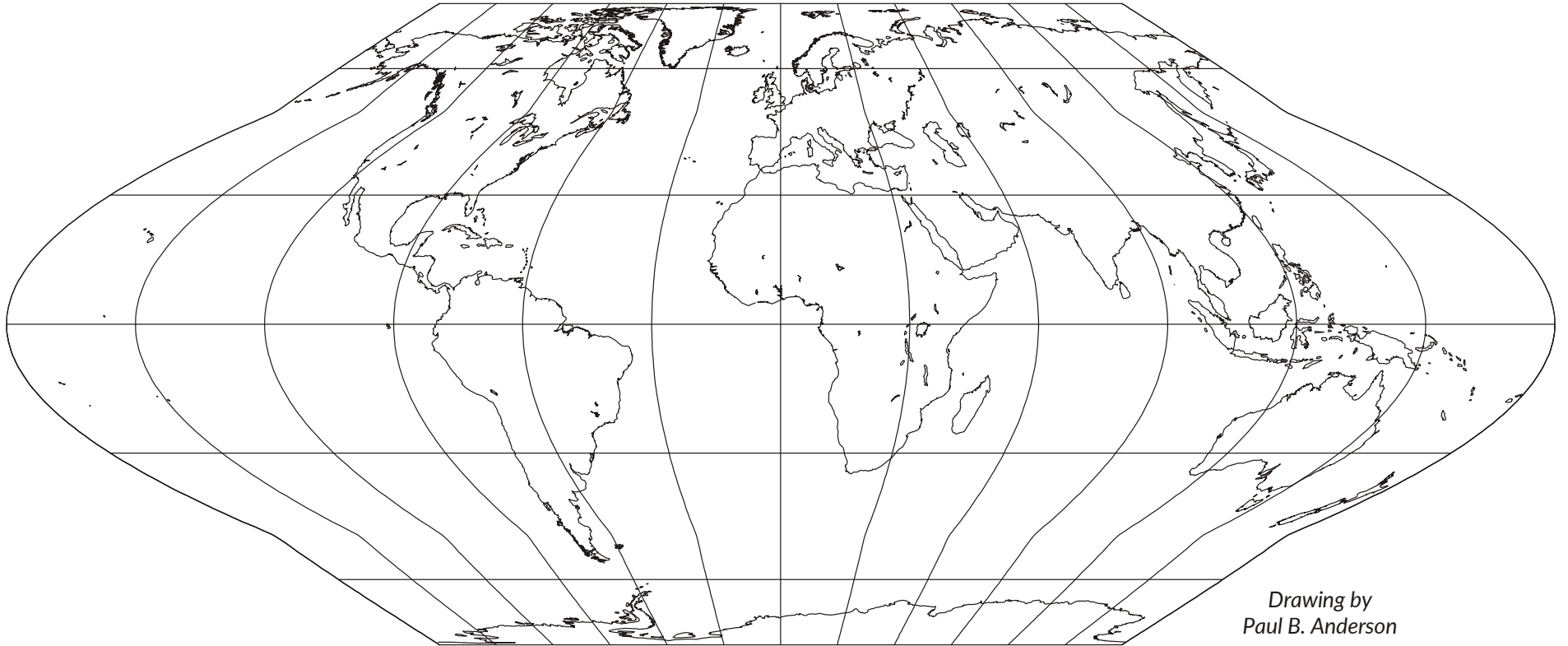
McBryde S2; (Fusion of Sinusoidal and Eckert VI); Pseudocylindrical; Equal-area; F. Webster McBryde; 1977
