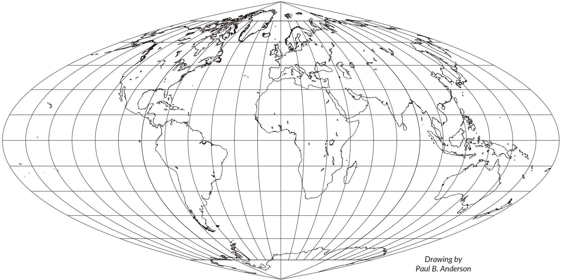
Siemon IV projection; Pseudocylindrical; Equal-area; Karl Siemon, 1937
